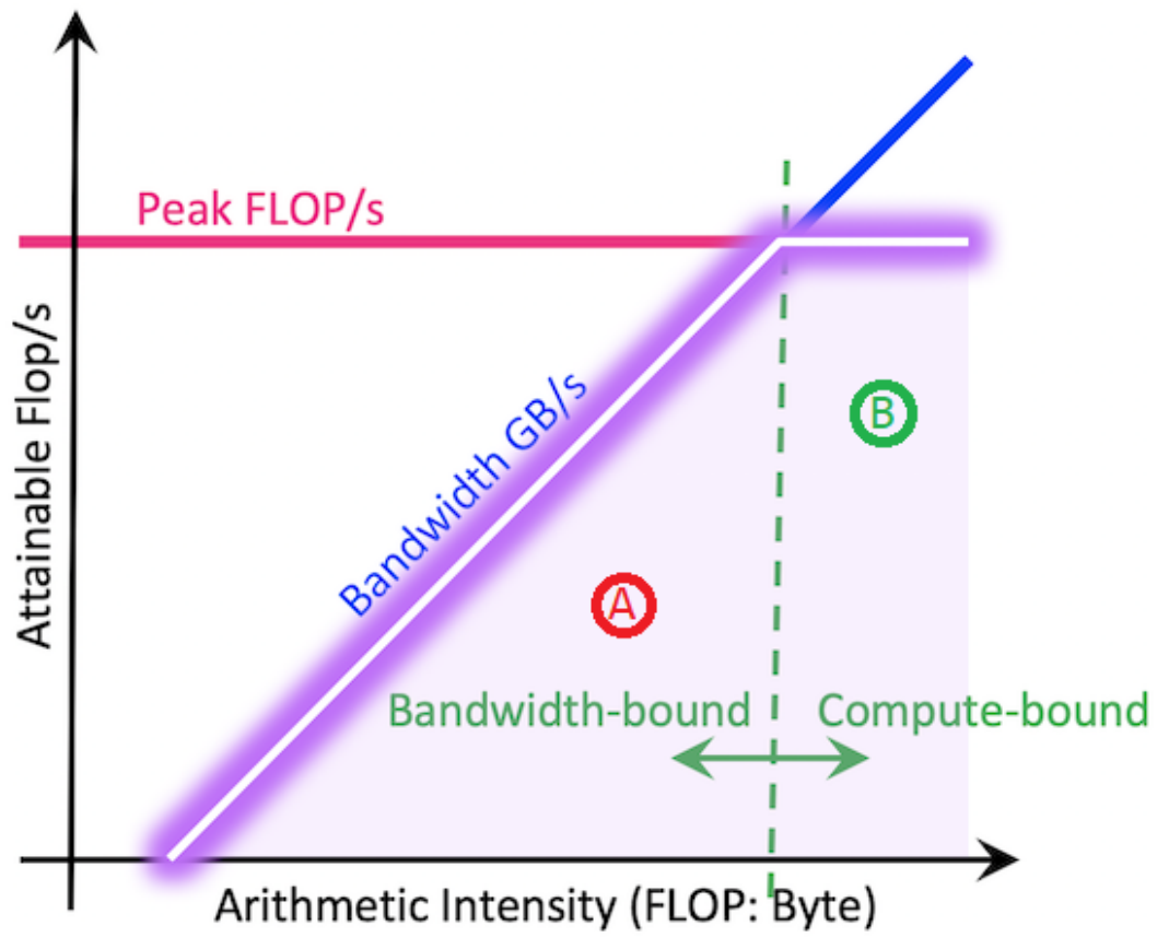
Figure 33: Roofline model. © Image taken from NERSC Documentation .
