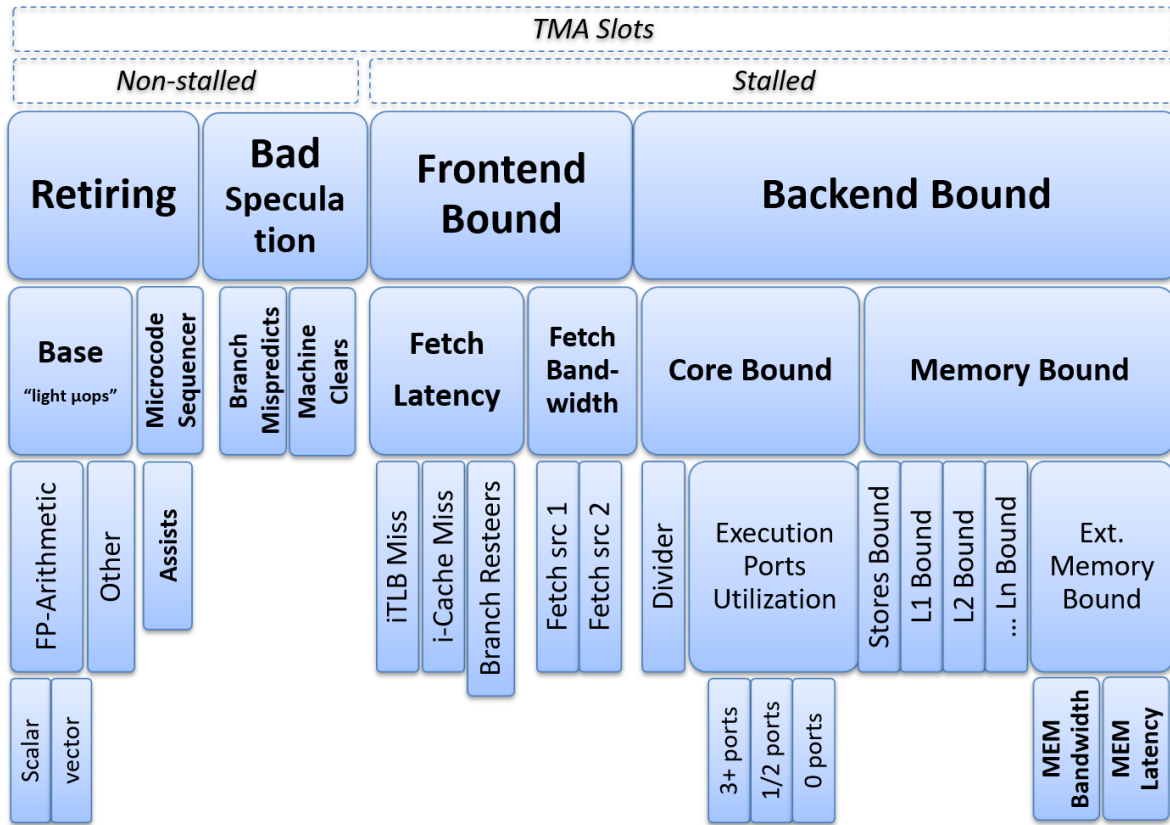
Figure 39: TMA 性能瓶颈的层次结构。© Image by Ahmad Yasin.
