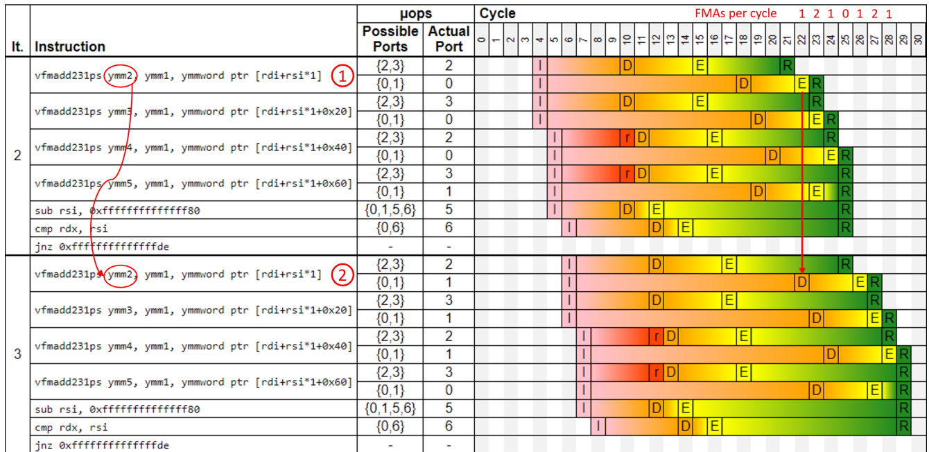
Figure 36: UICA pipeline diagram. I = issued, r = ready for dispatch, D = dispatched, E = executed, R = retired.
