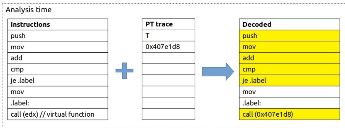
Figure 87: Intel 处理器跟踪解码
