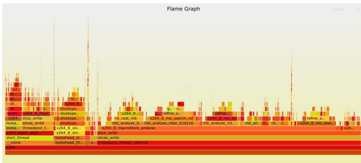
Figure 52: A Flame Graph for x264 benchmark.
