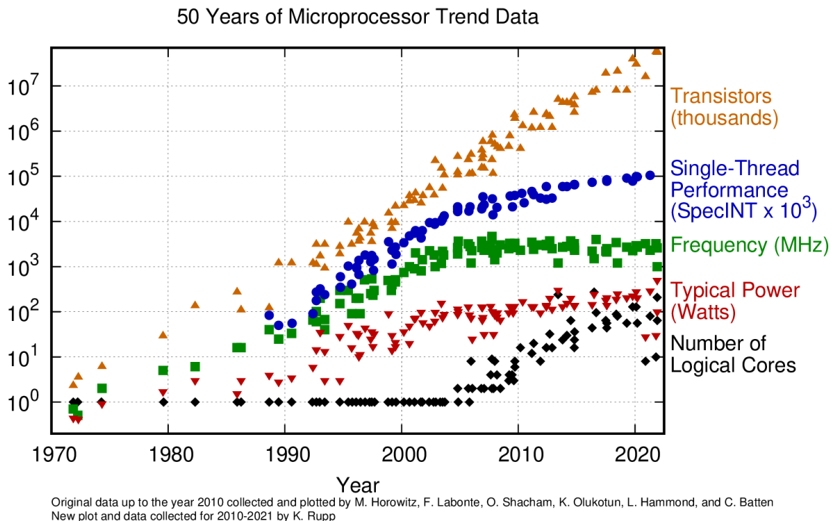
Figure 1: 50 Years of Microprocessor Trend Data. © Image by K. Rupp via karlrupp.net
