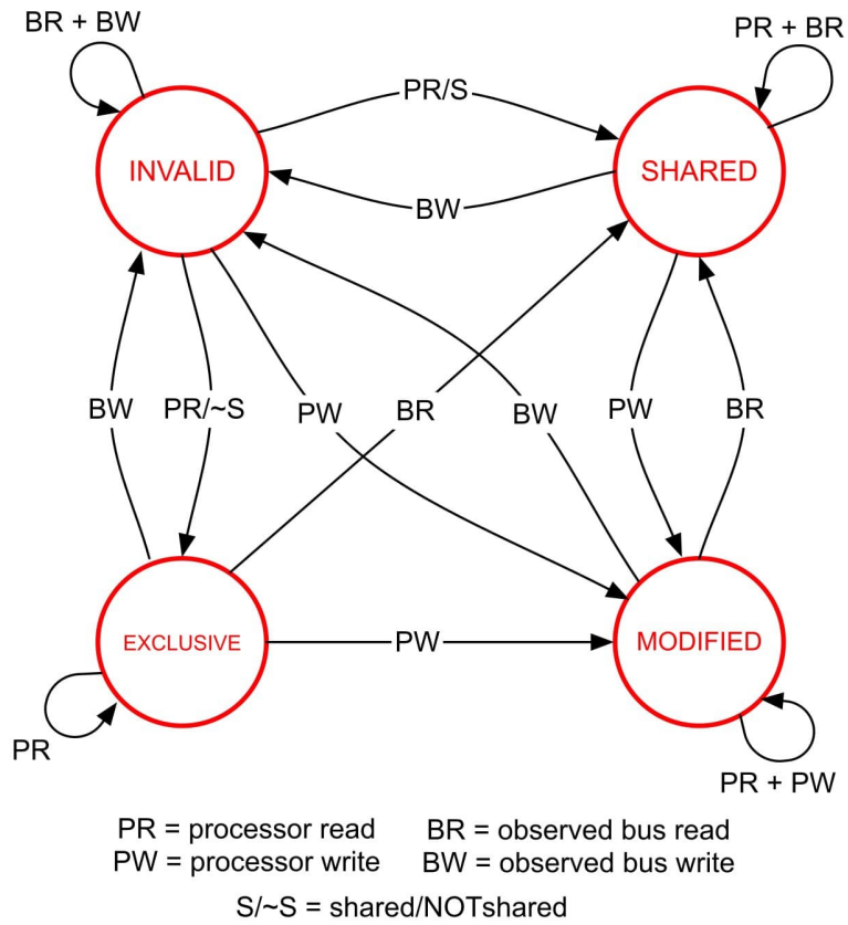
Figure 84: MESI 状态图. © Image by University of Washington via courses.cs.washington.edu.
