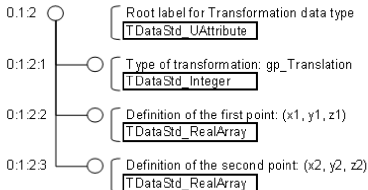
Figure 7: Data tree for translation
