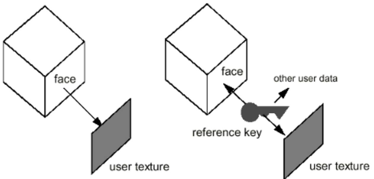
Figure 3: Topology driven versus reference-key driven approaches
