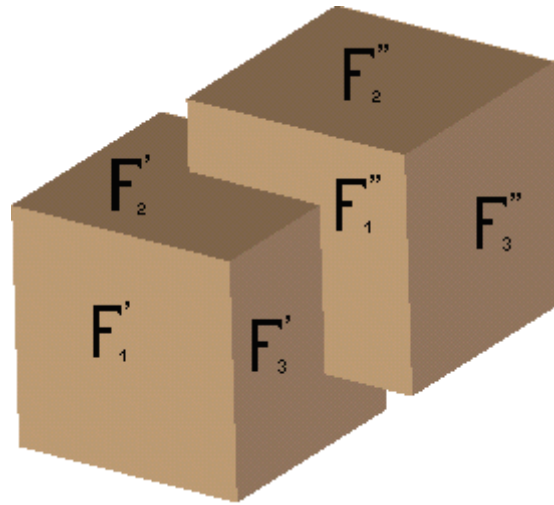
Figure 11: Resulting box
