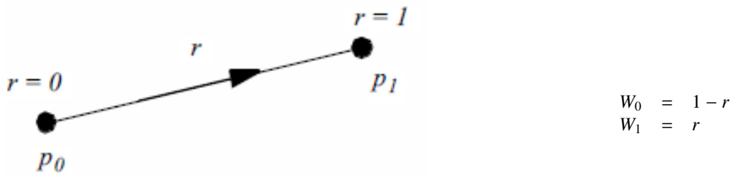
Figure 8.3: Parametric coordinate system and interpolation functions for a line.
