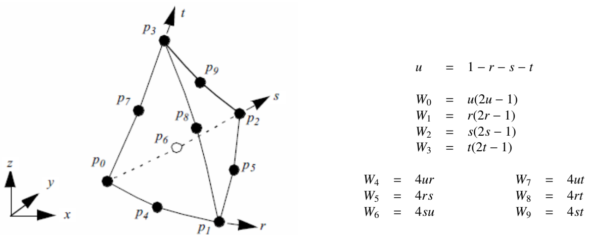
Figure 8.19: Parametric coordinate system and interpolation functions for a quadratic tetrahedron. In VTK parametric coordinates (r, s, t) run between (0, 1) , hence the coordinate system shift into the (\xi, \eta, \zeta) parametric system ranging from (-1, 1) .
