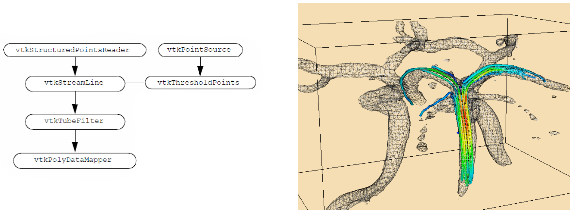
(CarotidFlow.cxx or CarotidFlow.py)
