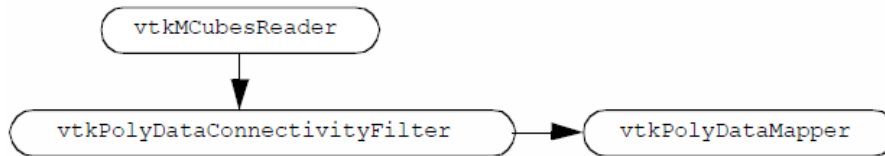
(b) Largest connected surface (PineRootConnectivity.cxx or PineRootConnectivity.py)
