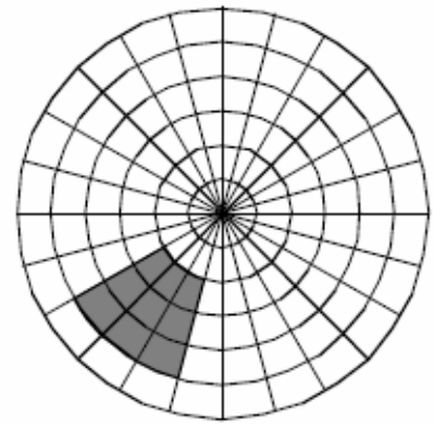
Polar coordinate grid (pie shaped region)
