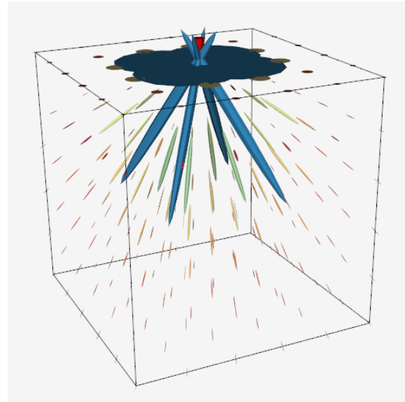
(b) Tensor ellipsoids. ( TensorEllipsoids.cxx or TensorEllipsoids.py )
