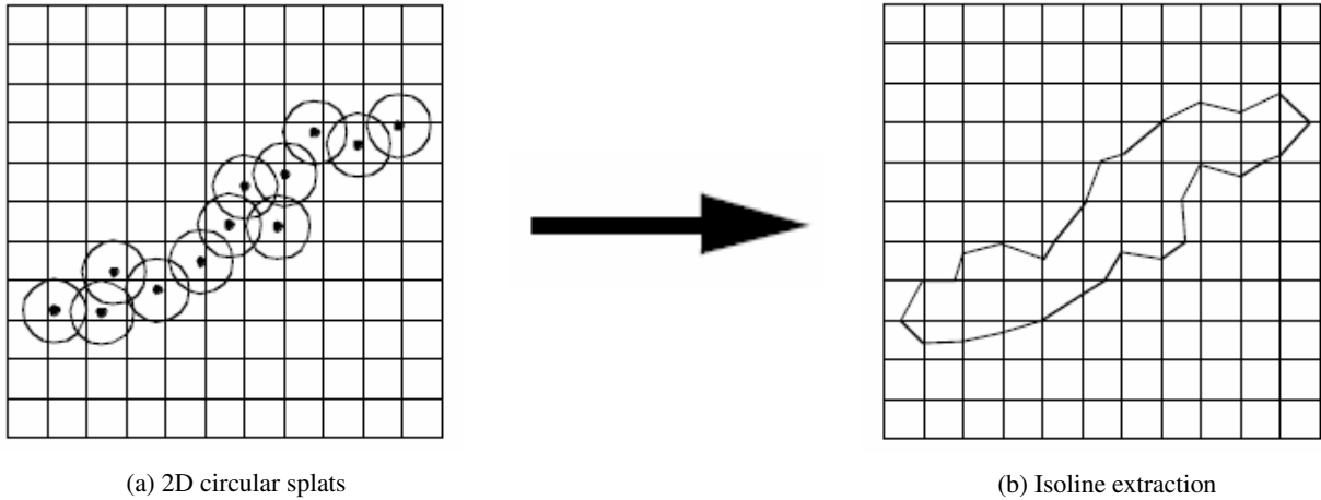
Figure 9.36: Splatting techniques depicted in 2D. (a) Injecting points into the image dataset (circular splats). (b) Visualizing the image dataset via contouring. Any image-based visualization technique could be used.
