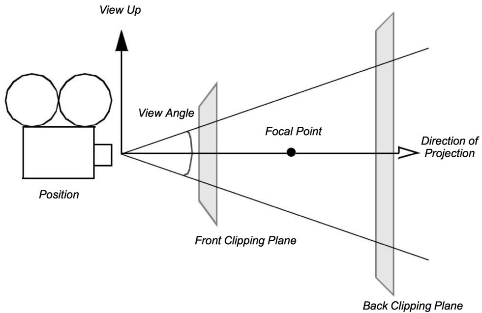
Figure 3.10: Camera attributes.
