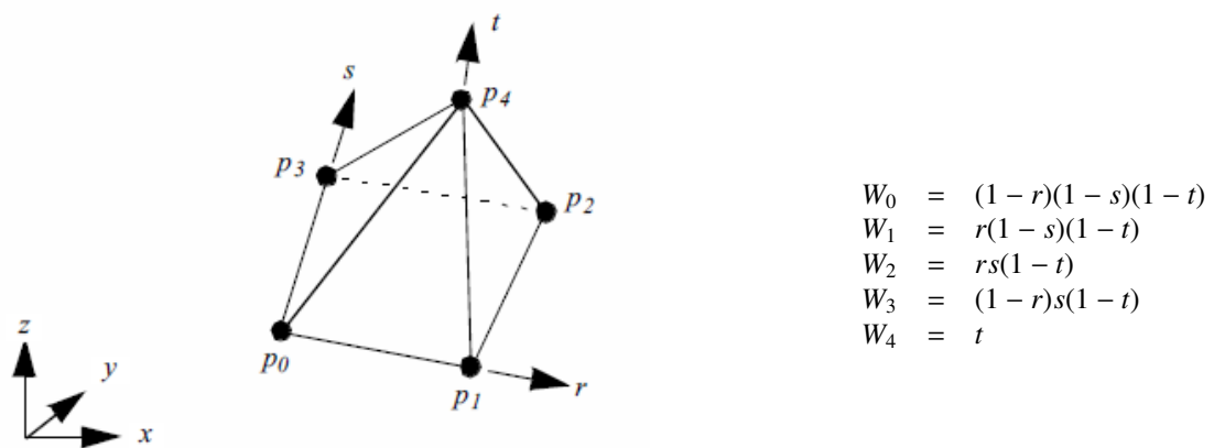
Figure 8.13: Parametric coordinate system and interpolation functions for a pyramid.
