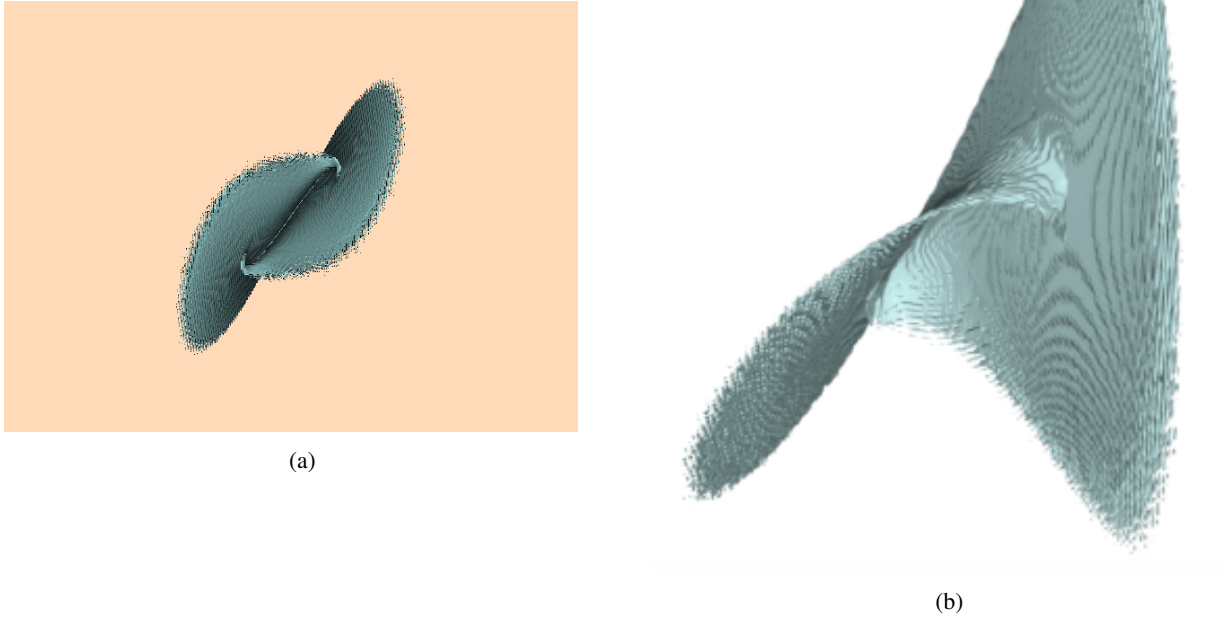
Figure 6.25: Visualizing a Lorenz strange attractor by integrating the Lorenz equations in a volume. The number of visits in each voxel is recorded as a scalar function. The surface is extracted via marching cubes using a visit value of 50. The number of integration steps is 10 million, in a volume of dimensions 200^3 . The surface roughness is caused by the discrete nature of the evaluation function. ( Lorenz.cxx or Lorenz.py )
