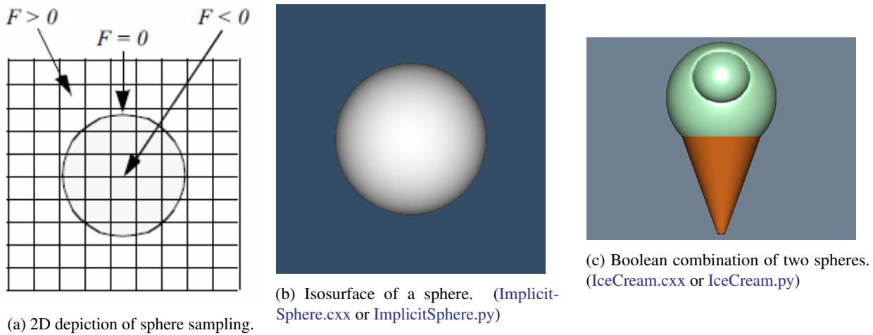
Figure 6.23: Sampling functions: (a) 2D depiction of sphere sampling] (b) Isosurface of sampled sphere; (c) Boolean combination of two spheres, a cone, and two planes. (One sphere intersects the other, the planes clip the cone).
