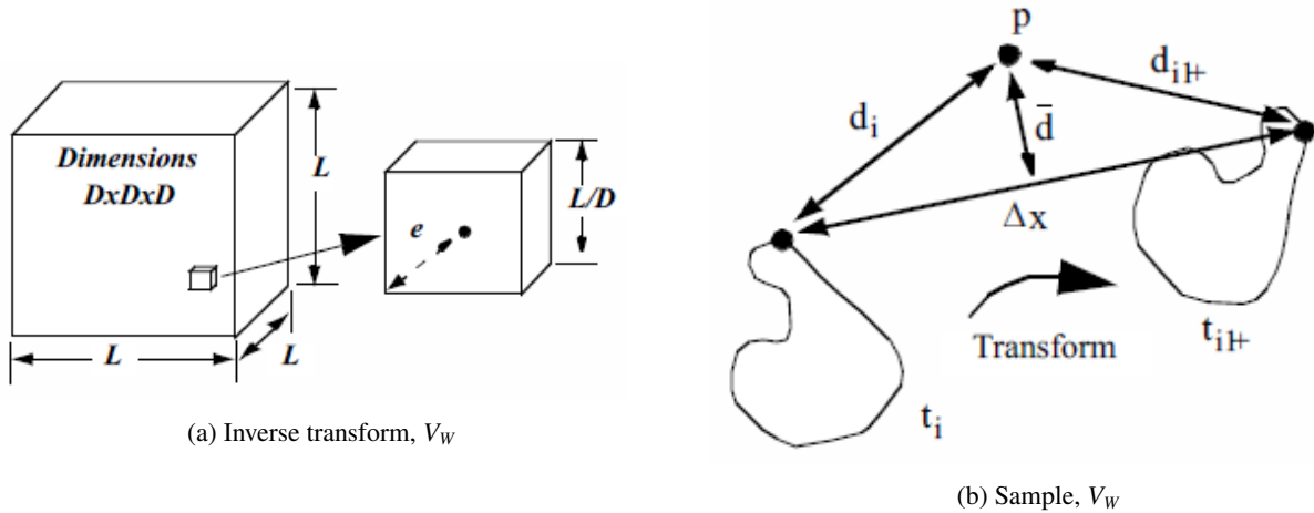
Figure 9.34: Computing sampling and stepping error.
